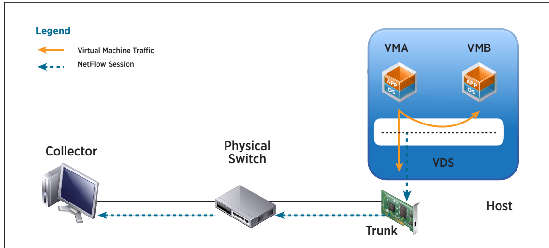
Figure 1. NetFlow Traffic
