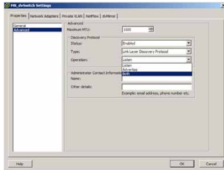
Figure 3. LLDP Configuration
